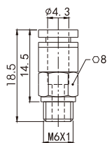
number : PC04-M6 Quick insertion air pipe joint
