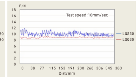
Frictional resistance comparison
