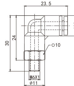
number: PL04-M6 Quick insertion air pipe joint
