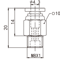
number: PC04-M8 Quick insertion air pipe joint
