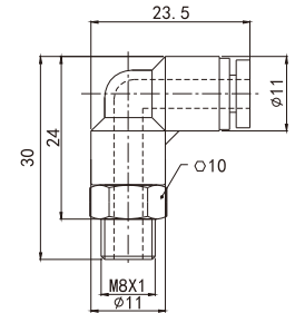
number: PL04-M8 Quick insertion air pipe joint
