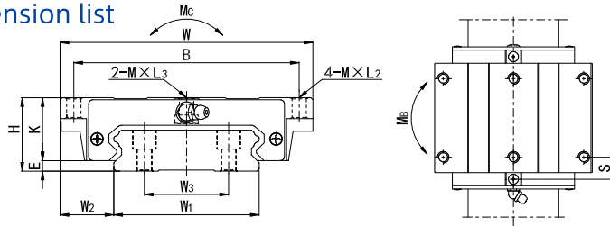
LGSW Series Dimension list Form: EA(flange type slider)
