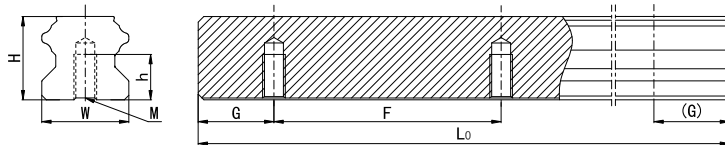
LGS series lower locking guide rail Dimension list
