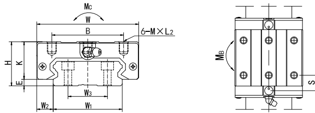
LGSW Series Dimension list Form: AA(Rectangular slider)
