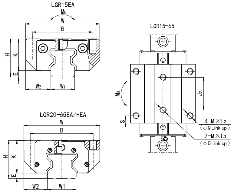
LGR series dimension list Form: EA(Screw hole type slider) HEA(Extended screw hole type slider)
