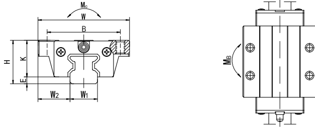
LGR12series dimension list Form: DE(Short screw hole slider) EA(Screw hole type slider) HEA(Extended screw hole type slider)
