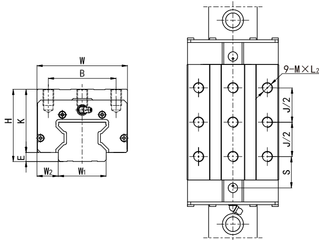
LGR series dimension list Form: AN(Thickened rectangular slider)
