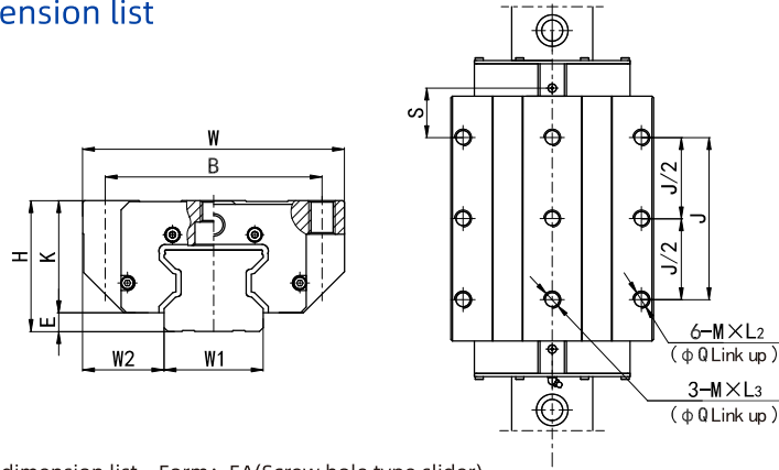
LGR series dimension list Form: EA(Screw hole type slider)
