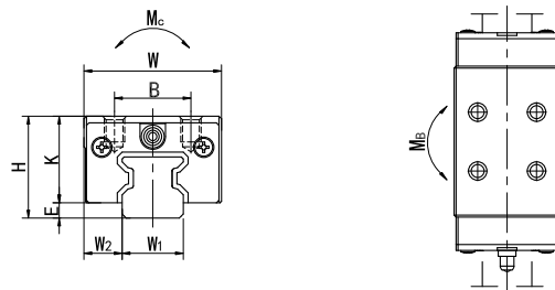
LGR12series dimension list Form: DN(Short rectangular slider) AN(Thickened rectangular slider) HAN(Extended and thickened rectangular slider)
