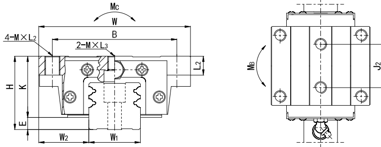
LG EAX,HEAX series(Specific rigid reinforcement type)
