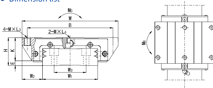
LGW25EA series dimension list Form: EA(flange slider) SEA(short series)
