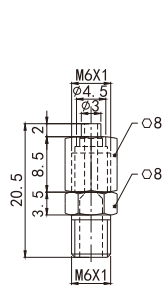
number: \phi 4-M6 Flared straight joint
