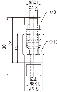
number: \phi 4-M8 Copper pipe straight joint
